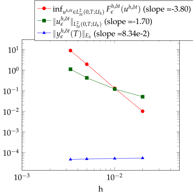
FIGURE IV.2: Minimal value of the functional F^{h,\delta t}_\epsilon in L^2_{\delta t}(0,T;U_h) , norm of the control \|u^{h,\delta t}_\epsilon\|_{L^2_{\delta t}(0,T;U_h)} , and distance to the target \|y^{h,\delta t}_\epsilon(T)\|_{E_h} in Case (b).
