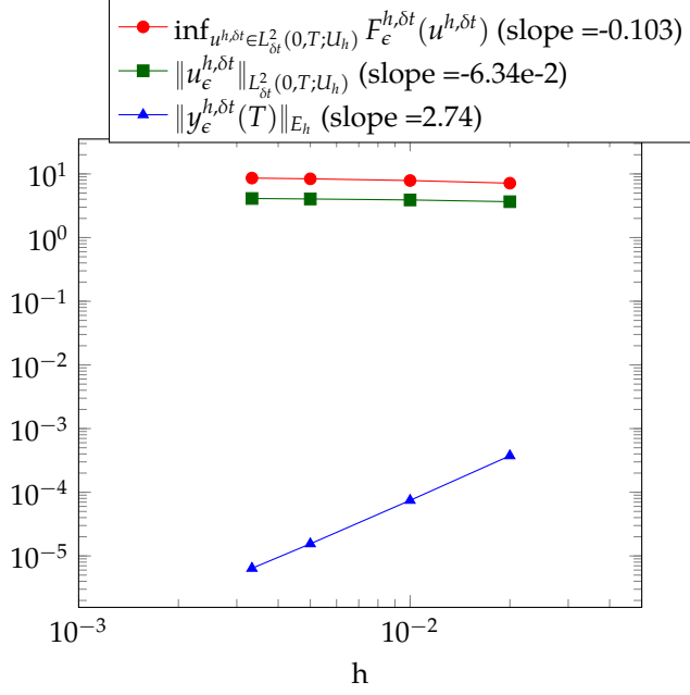
FIGURE IV.1: Minimal value of the functional F^{h,\delta t}_\epsilon in L^2_{\delta t}(0,T;U_h) , norm of the control \|u^{h,\delta t}_\epsilon\|_{L^2_{\delta t}(0,T;U_h)} , and distance to the target \|y^{h,\delta t}_\epsilon(T)\|_{E_h} in Case (a).
